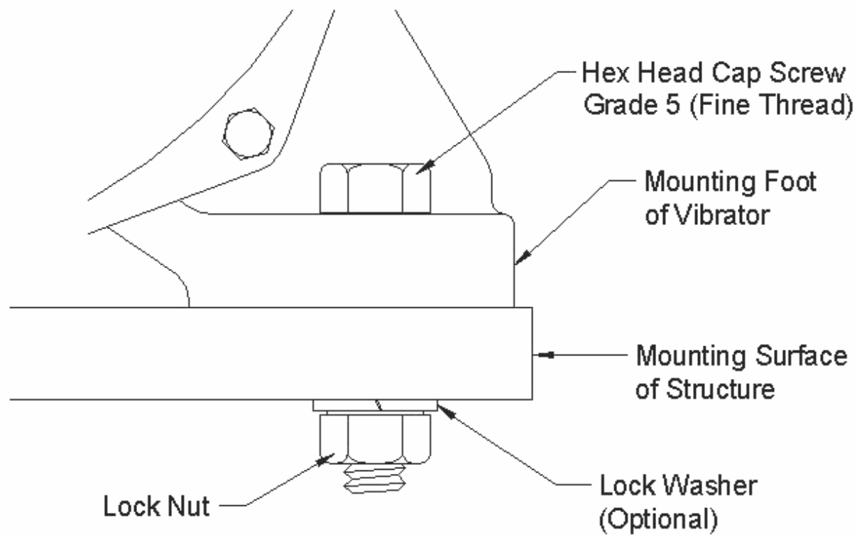
Vibrator Mounting Arrangement
